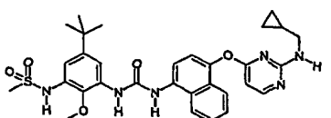
N-[5-tert-Butyl-3-(3-{4-[2-(cyclopropylmethyl-amino)-pyrimidin-4-yloxy]-naphthalen-1-yl]-ureido)-2-methoxy-phenyl]-methanesulfonamide;
